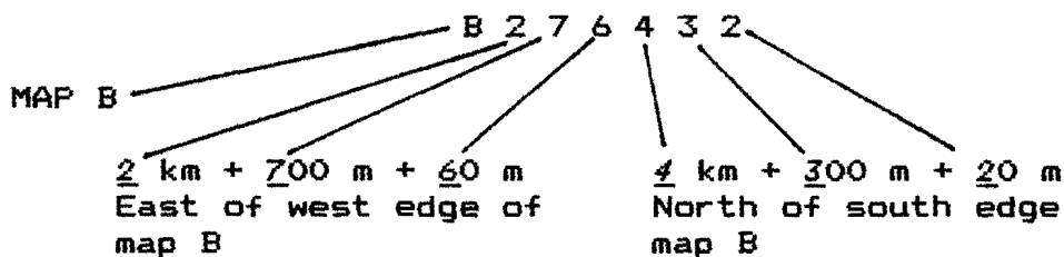
Figure 2. Sample 7-figure coordinate group. This coordinate group plots a position to lie within a 10 meter square centered on the point described.
