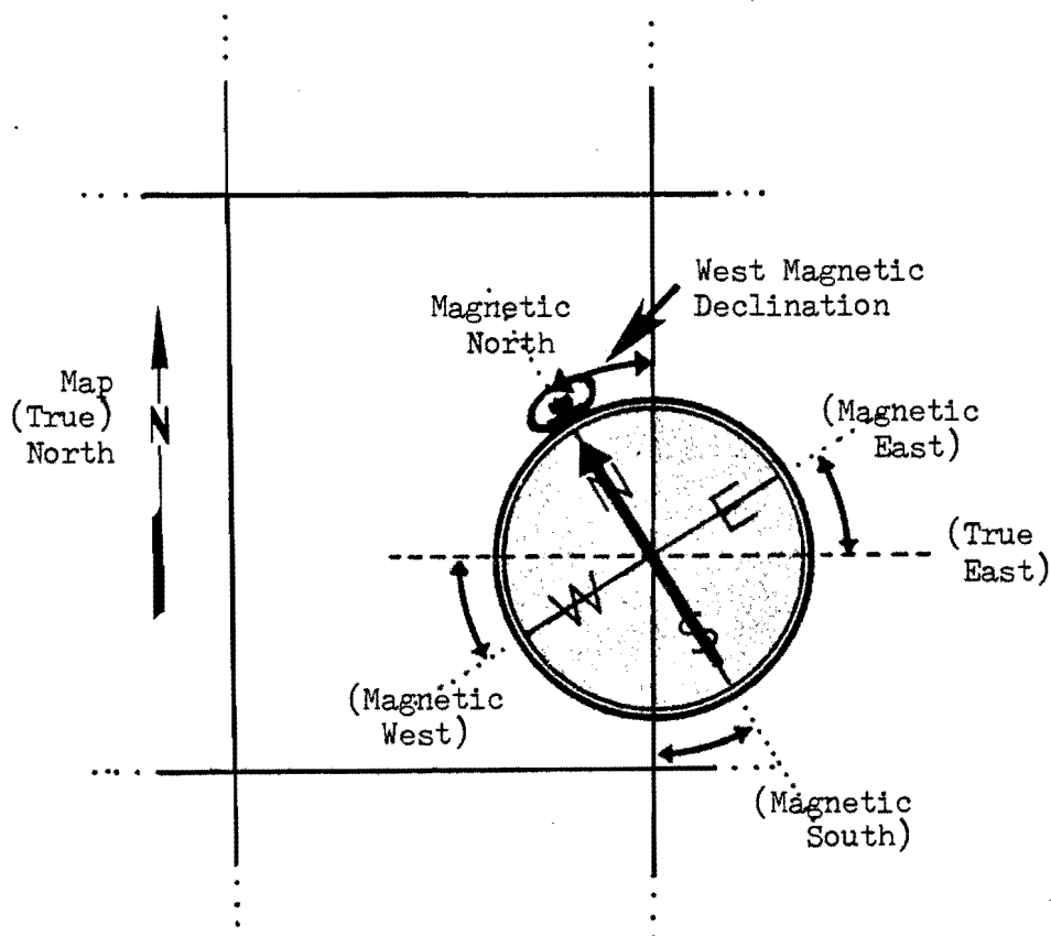
FIGURE 8-5: Magnetic Declination
