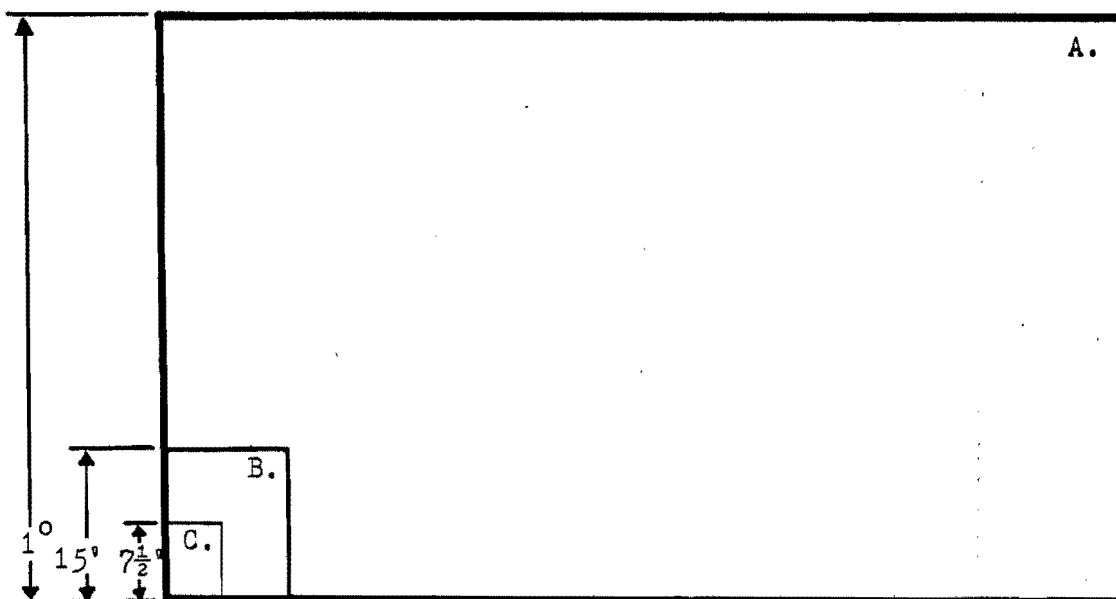
FIGURE 8-3: Relative Coverage of 3 USGS Topographic Map Series Sizes. A: 1:250,000 Series ( 1^{\circ} x 2^{\circ} ) B: 15' x 15' Quadrangle Series (1:62,500) C: 7'30" x 7'30" Quadrangle Series (1:24,000)
