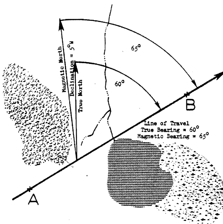
FIGURE 8-11: Declination correction
