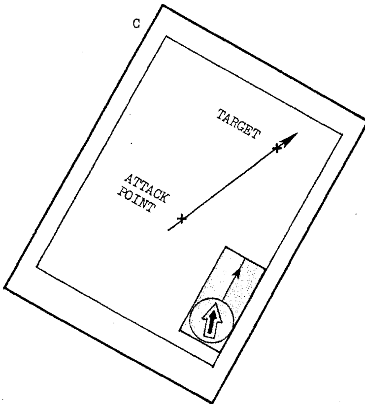
FIGURE 8-12: Map and compass method for determining bearings (continues on next page)
