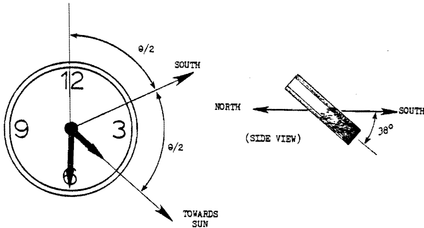
FIGURE 8-19: Watch and sun method of determining direction
