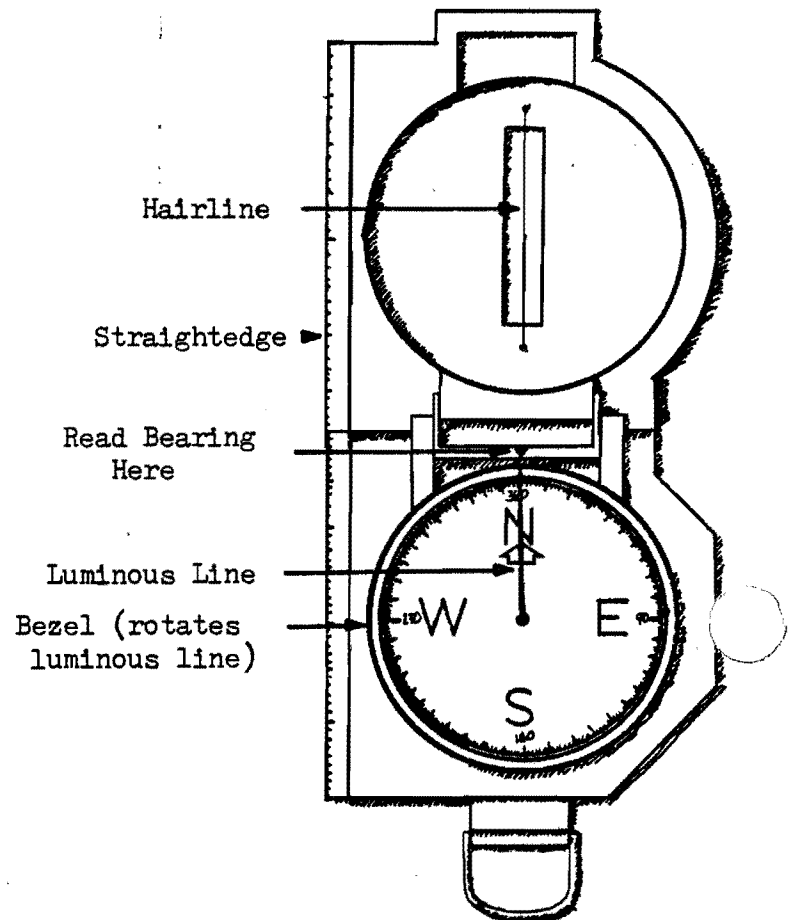
FIGURE 8-7: The Lensatic Compass
